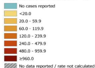
14-day COVID-19 case notification rate per 100 000 weeks 47 - 48
