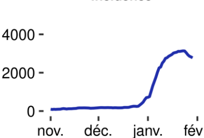
Incidence
