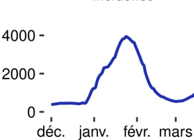
Incidence
